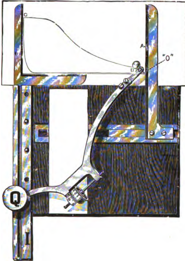
FIG. 310.—Method of Averaging a Diagram with one Type of Planimeter. The pin, Q , is set in the groove, I . The card is held on the board between clamps, C and A . The tracing point, O , is set at point, D , and the arm moved clockwise, the vernier and drum having been set at zero.
